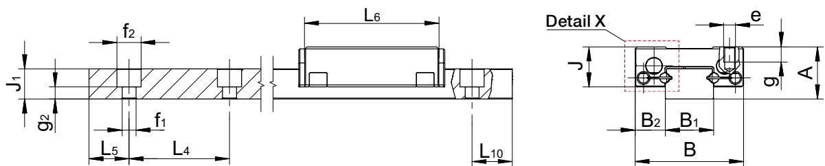
Detail X
